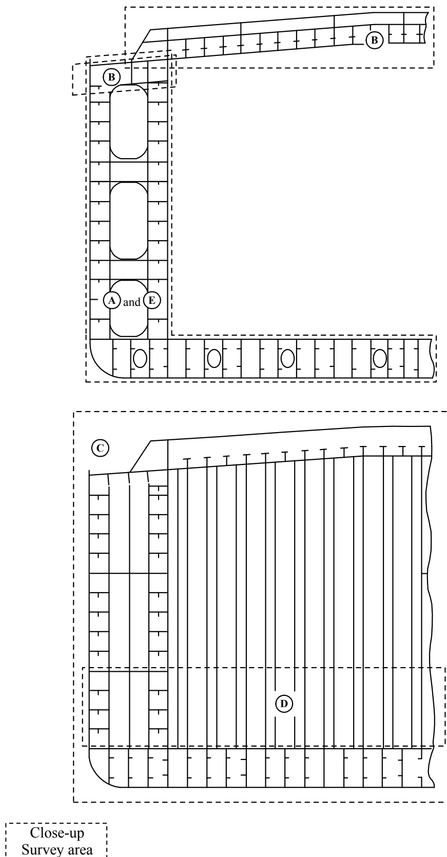
FIGURE 9 Thickness Measurement – Chemical Carriers
