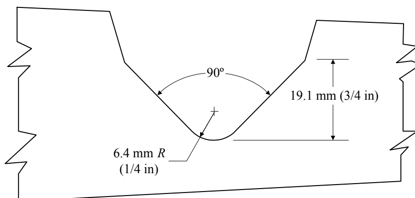
FIGURE 8 Typical Deep Groove Preparation for Welding Repair
