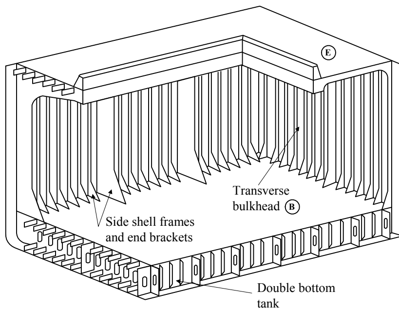
FIGURE 4 Areas for Close-Up Survey of General Dry Cargo Ships (2004)
