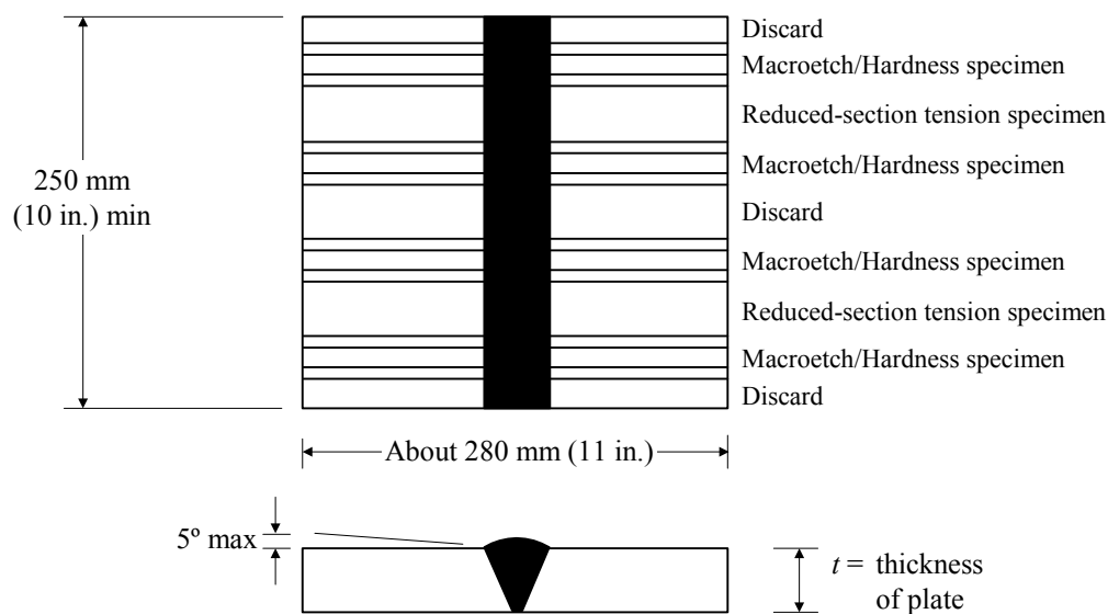
FIGURE 10 Welding Qualification Test Plate Location of Test Specimens (2009)
