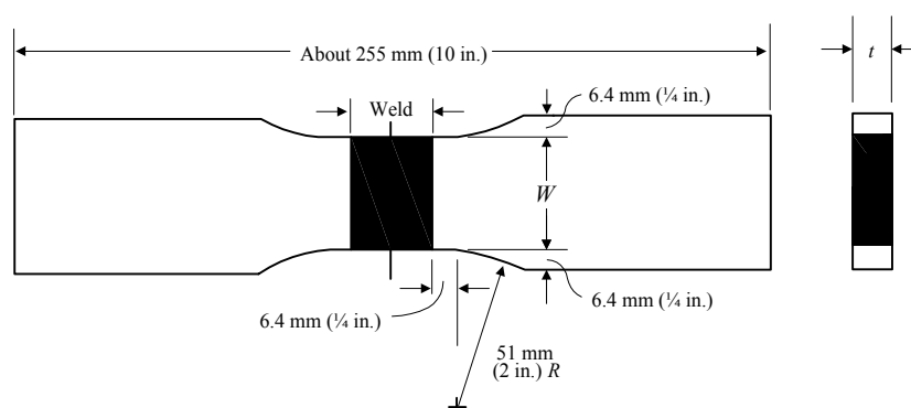
FIGURE 11 Reduced-section Tension Specimen (2009)
